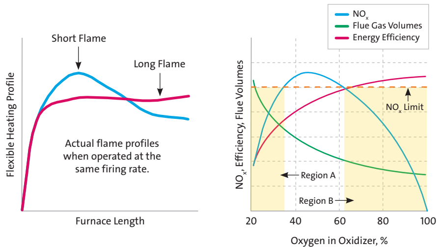
Figure 1: Flexible heating profile (left) and low NO x operation (right)
